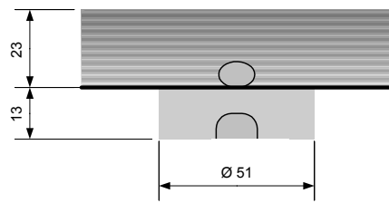
Mounting with wall switch box
